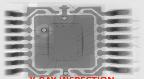
X-RAY INSPECTION
